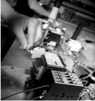
Sub Assembly wiring and continuity testing
